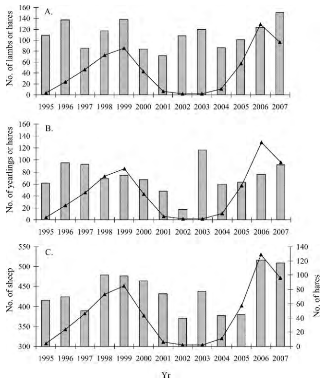
Figure 2. Numbers of Dall’s sheep lambs (A), yearlings (B), and adults (C) recorded on aerial surveys during mid-June (bars) and counts of snowshoe hares (triangles and solid line) in the central Alaska Range, USA, 1995–2007.
