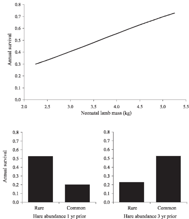
Figure 3. Effects of changes in parameter values on survival estimates for Dall's sheep lambs in the central Alaska Range, USA, 1995–2007. We estimated survival using a model with the covariates neonatal lamb mass and hare abundance estimated 1 year and 3 years previously. Each graph depicts survival estimated across the observed range of values of one parameter with all others held constant.
