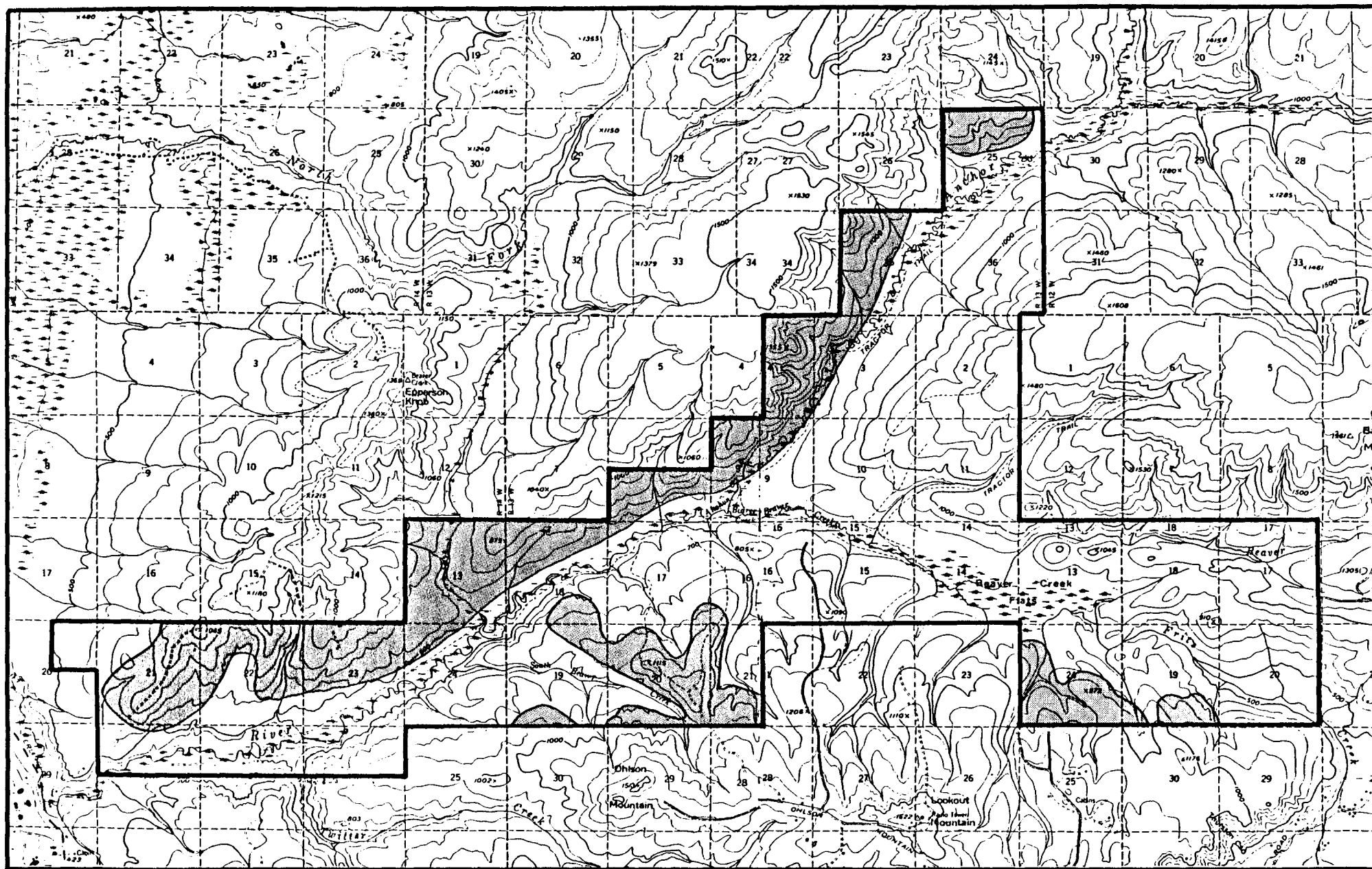
PLATE 1. DISTRIBUTION OF COAL BEARING KENAI GROUP SEDIMENTS IN THE ANCHOR RIVER-FRITZ CREEK CRITICAL HABITAT AREA
