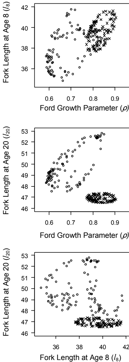
Figure 7. Scatterplots of bootstrapped 95% confidence regions for von Bertalanffy parameter estimates, Alaska Peninsula Area female (o, n = 50) and male (x, n = 218) black rockfish. Plots are parameter values for the 100 replicates most distant from the bootstrap mean.
