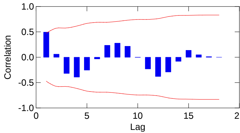
Autocorrelation Plot
