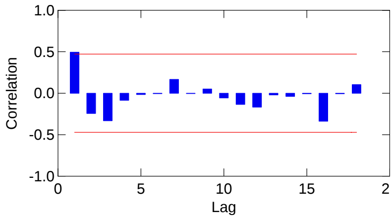
Partial Autocorrelation Plot
