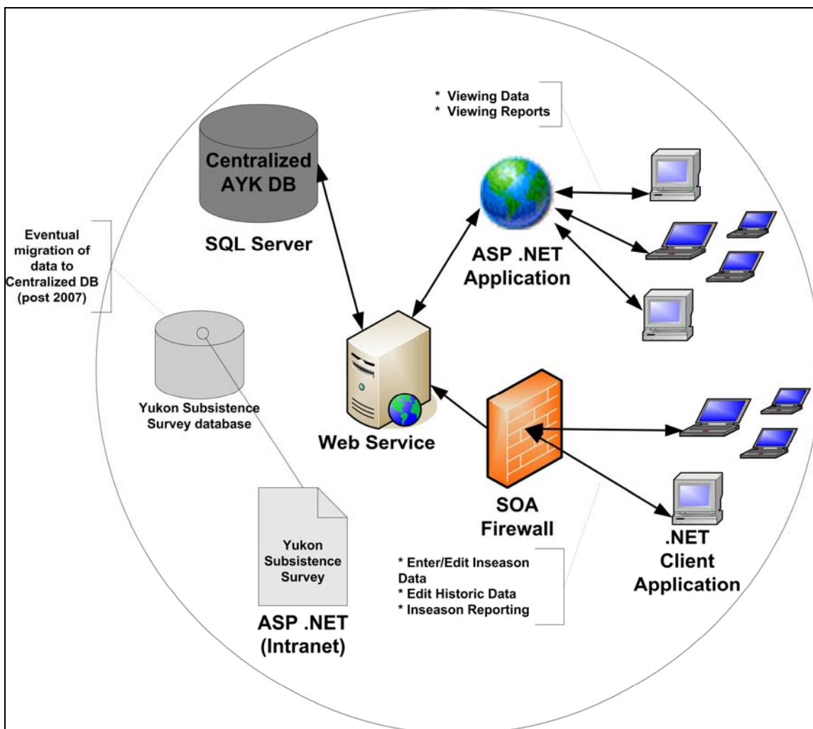
Figure 6. —Final relationship among components of the AYK salmon database management system.
