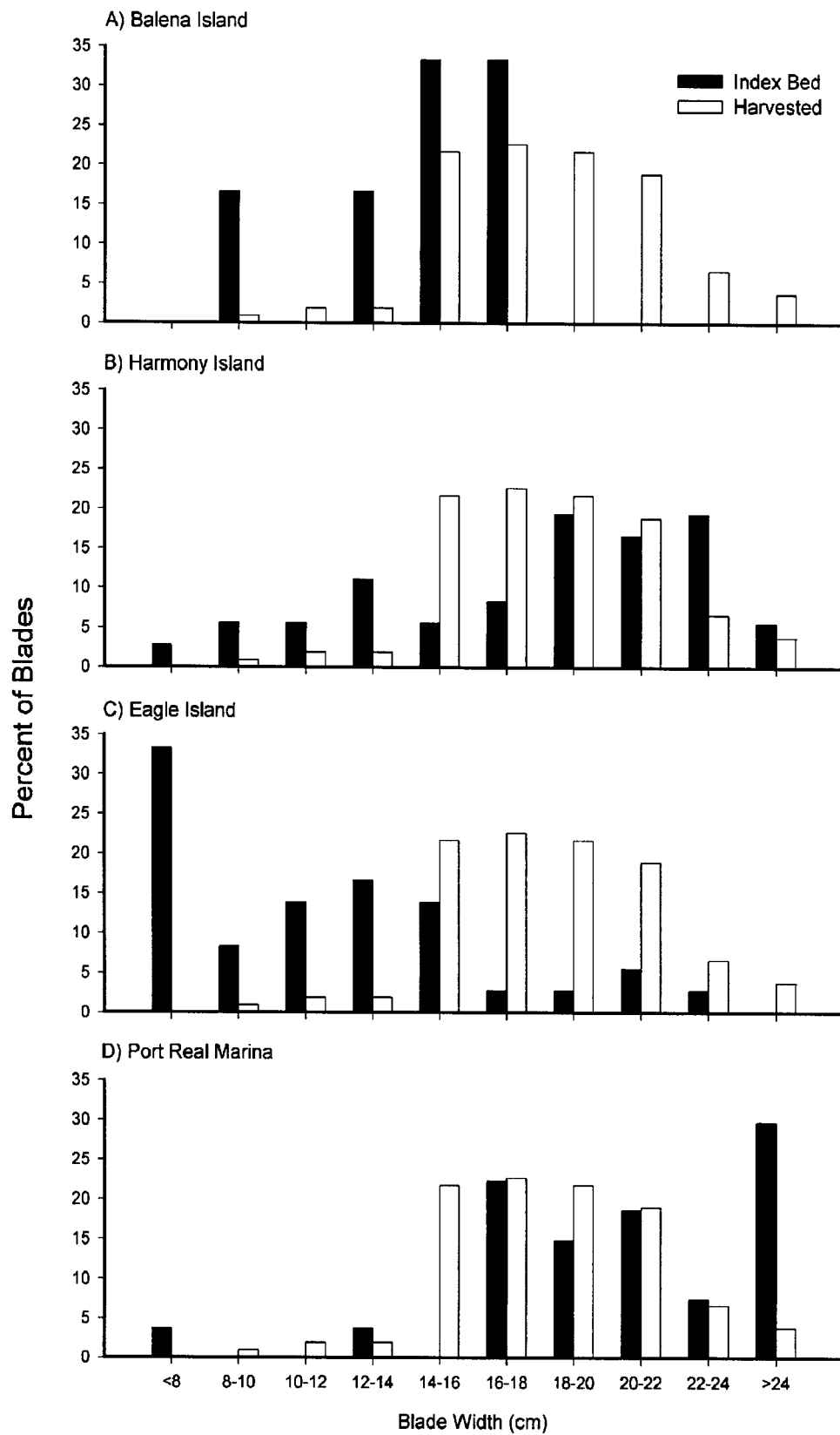
Figure 4. Size distribution of Macrocystis blade widths at the index beds compared to the harvested kelp.
