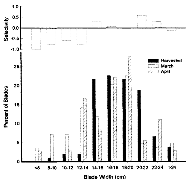
Figure 3. The proportion of Macrocyrtis blades of various widths of harvested kelp, kelp in the Port Alice bed before harvest (March), and later in the spring (April). Selectivity indices for the different blade widths using the harvested and March data are shown in the upper graph. Negative and positive selectivity indices indicate avoidance and selection, respectively.
