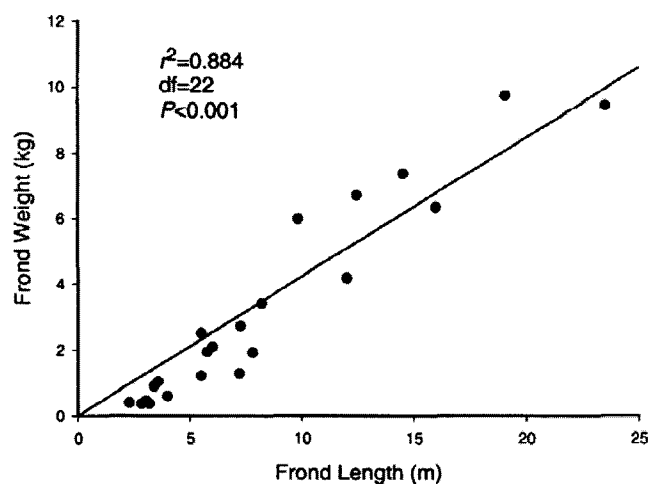
Figure 2. The relationship between Macrocystis frond length and weight. The results of the regression analysis are also shown.
