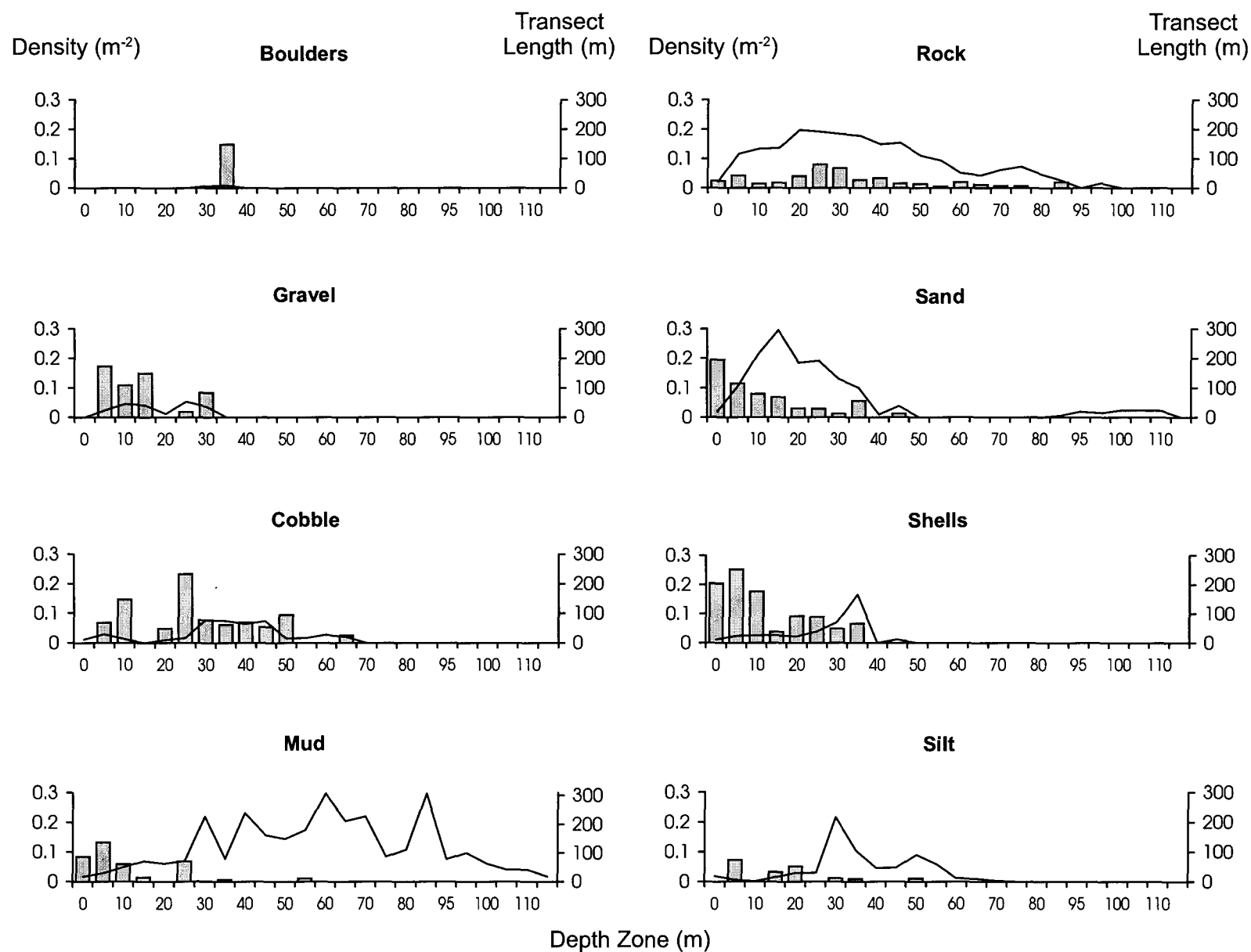
Figure 3. Density of P. californicus (bars) and transect lengths (lines) in 5-m depth zones for each of 8 substrate types. Transect lengths are the total of lengths of the survey paths in each of the substrate types.
