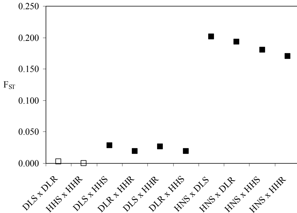
Figure 14. —Estimates of F_{ST} for all population pairs. Black squares (■) denote statistically significant ( P < 0.05 ) genetic differentiation based on a G -test of genotypic frequency homogeneity. Population abbreviations are Dickey Lake steelhead (DLS), Dickey Lake rainbow trout (DLR), Hungry Hollow Creek steelhead (HHS), Hungry Hollow Creek rainbow trout (HHR), Hanagita Lake steelhead (HNS).
