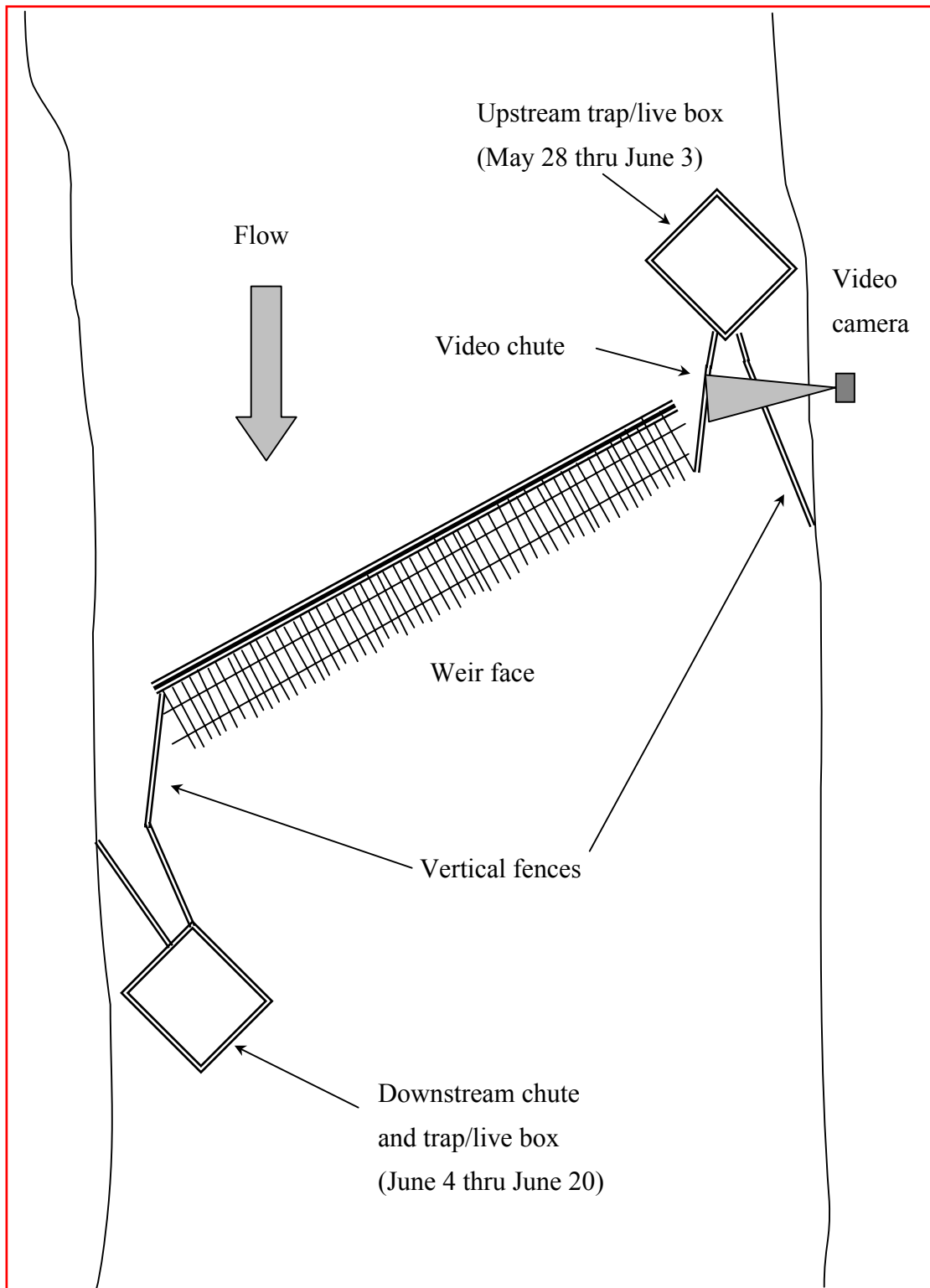
Figure 5. —Schematic of weir configuration used at Dickey Lake in 2001.
