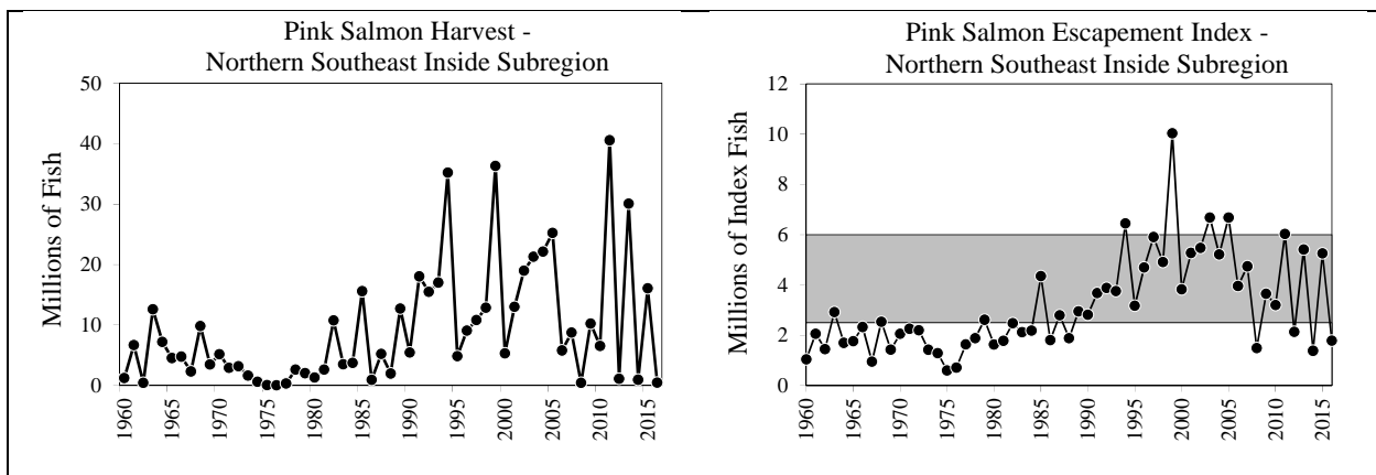
Figure 4.—Annual pink salmon harvest and escapement index for the Northern Southeast Inside Subregion, 1960–2016. The shaded area shows the escapement goal range of 2.5 to 6.0 million index spawners.
