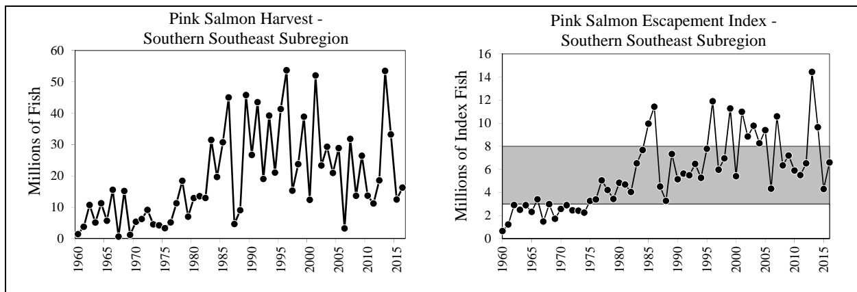
Figure 3.—Annual pink salmon harvest and escapement index for the Southern Southeast Subregion, 1960–2016. The shaded area shows the escapement goal range of 3.0 to 8.0 million index spawners.
