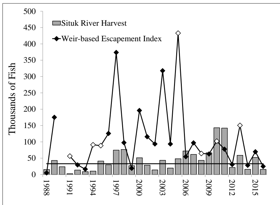
Figure 2.—Annual Situk River pink salmon harvest and weir-based escapement index for the Situk River, 1988–2016. The horizontal black line shows the lower-bound sustainable escapement goal of 33,000 pink salmon counted through the weir by 5 August. Black squares represent years when the weir was operated through 5 August and white squares represent years when the weir was pulled early and the escapement through 5 August was estimated.
