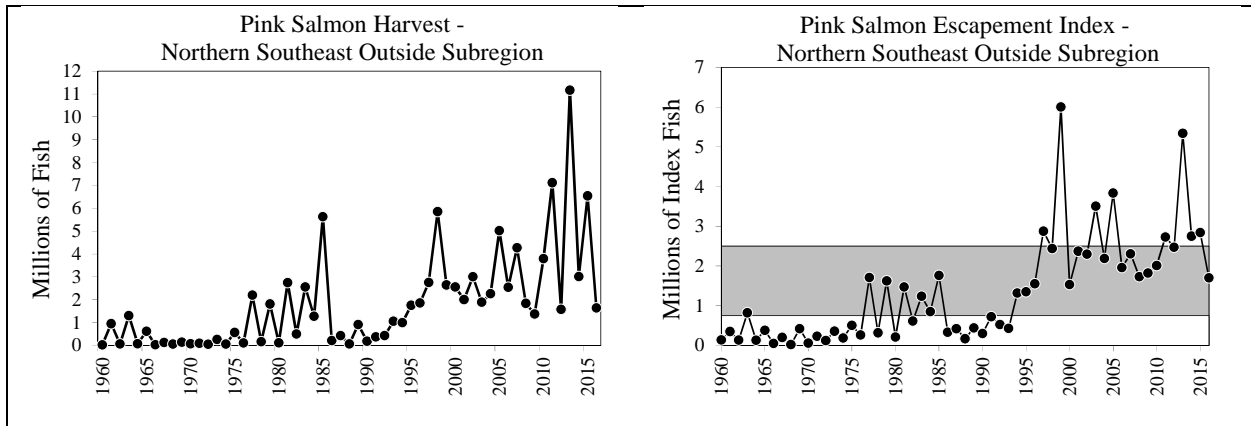
Figure 5.—Annual pink salmon harvest and escapement index for the Northern Southeast Outside Subregion, 1960–2016. The shaded area shows the escapement goal range of 0.75 million to 2.5 million index spawners.
