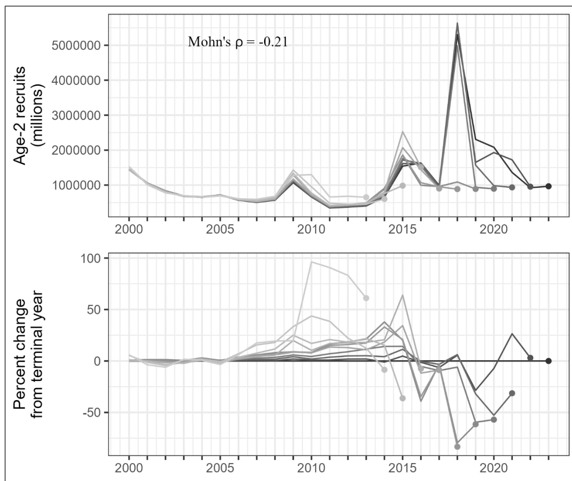
Figure 25.—Mohn's \rho and retrospective peels of sablefish recruitment for the last nine years.
