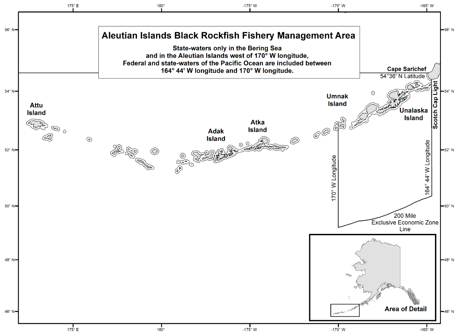
Figure 3.—Aleutian Islands state-waters black rockfish management area.
