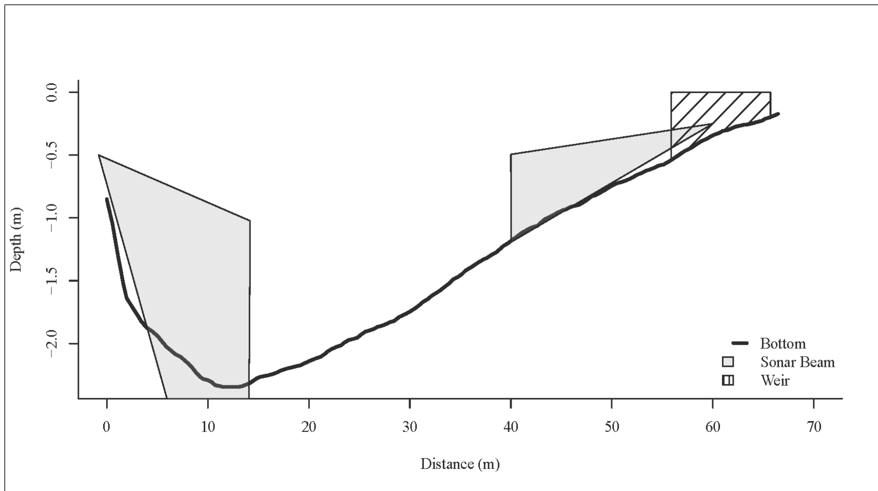
Figure 5.—Depth profile of the Sheenjek River and approximate sonar ranges at the Sheenjek River sonar project, August 4, 2024.
