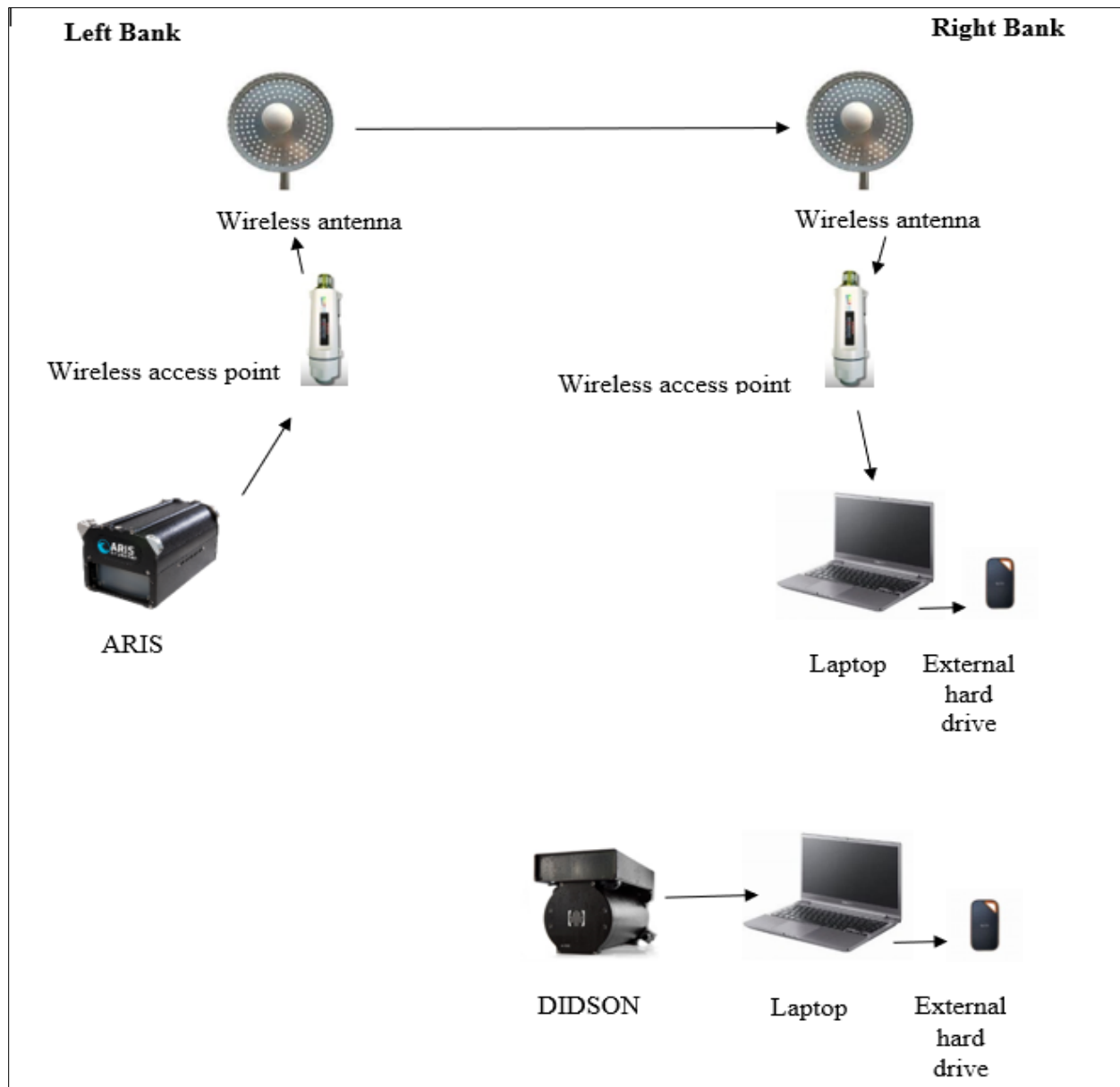
Figure 3.—ARIS (adaptive resolution imaging) and DIDSON (dual-frequency identification) sonar equipment schematic at the Sheenjek River sonar project, 2024.
