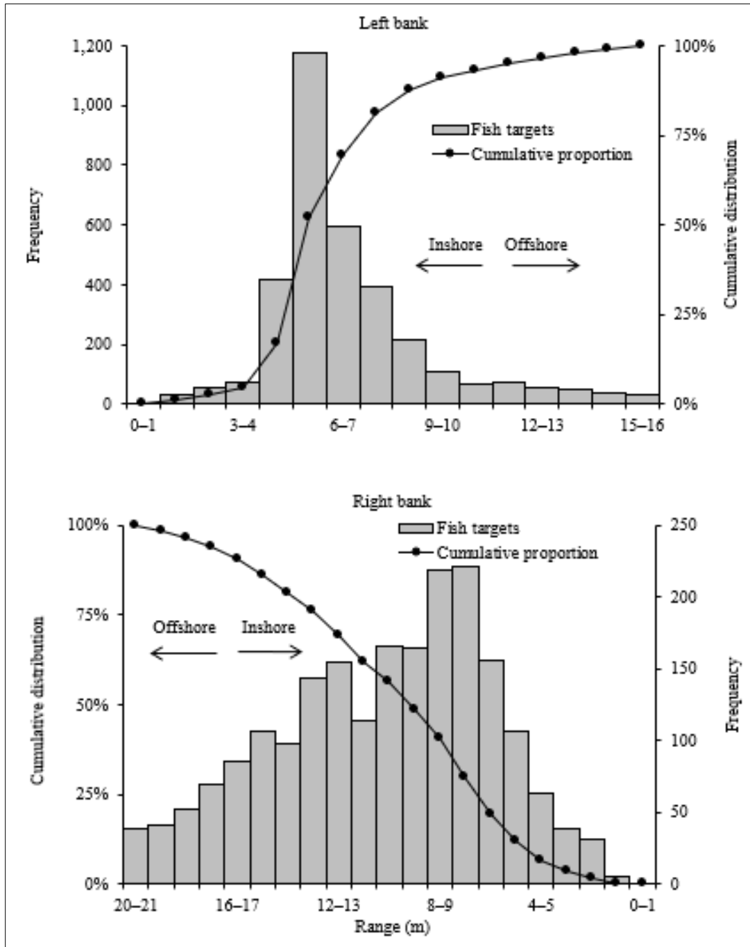
Figure 7.–Left- and right-bank horizontal distribution of unexpanded fish targets at the Sheenjek River sonar project, August 5–September 25, 2024.
