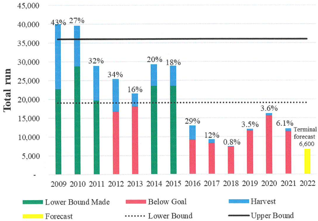
Taku River Chinook Salmon Escapement and Harvest, 2009 to 2021.
