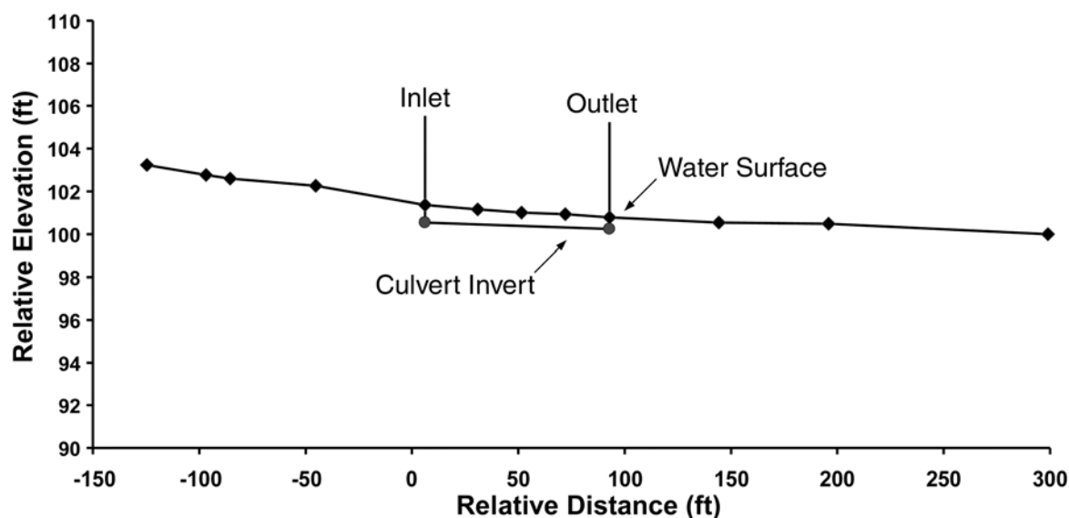
Figure 13. Water surface and culvert invert profiles for No-Name Creek September 13, 1997.
