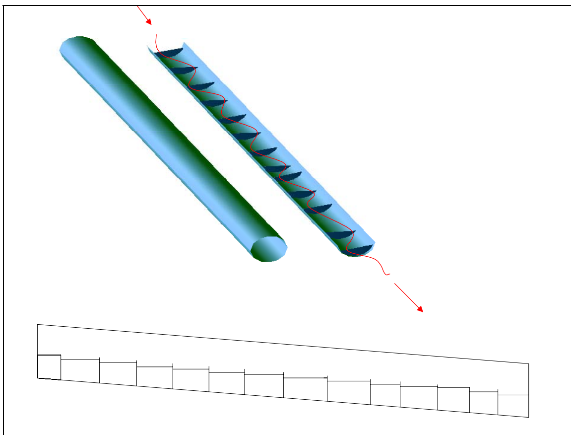
Figure 18. Schematic of Soldotna Creek culvert showing the pattern of flow through culvert and the placement of 13 baffles.
