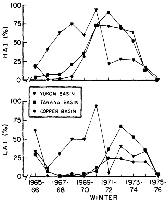
Figure 2. Snowshoe Hare Abundance Indices (HAI) and Lynx Abundance Indices (LAI) for three regions of Alaska, 1965-66 through 1975-76. Indices were calculated from trapper questionnaire responses with methods by Brand and Keith (1979). (Indices of 0-19% = scarce, 20-50% = intermediate, and 51-100% = abundant).
