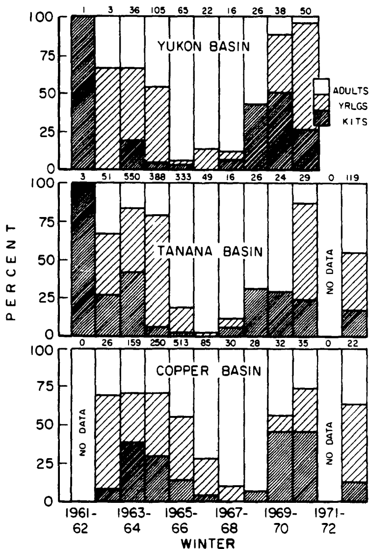
Figure 5. Age distribution of 3,130 female lynx carcasses collected from three regions of Alaska, 1961-62 through 1972-73 (kits = 0-12 months, yearlings = 13-24 months, and adults = 25+ months). Annual sample sizes are noted above the figure for each region.
