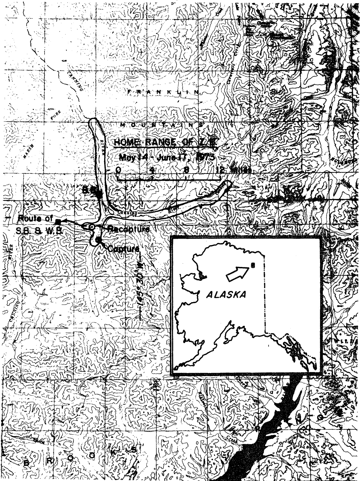
Fig. 1. Home range of grizzly bear "Z.B.", May 14-June 17, 1973. S.B., W.B. and B.B. = other grizzlies found in the area.
