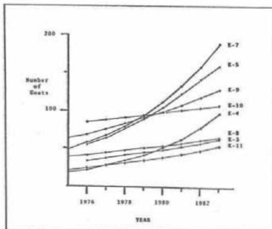
Figure 3. Trends in 8 mountain goat populations near Ketchikan, Alaska, 1975 - 1983
