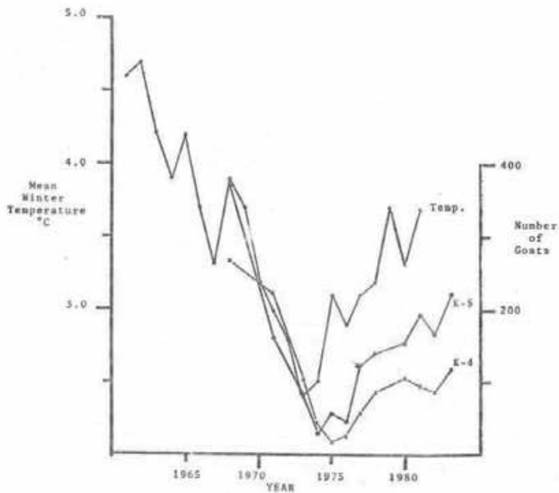
Figure 6. Trends in mean winter temperature at Ketchikan, Alaska and 2 nearby mountain goat populations, 1960 - 1983.
