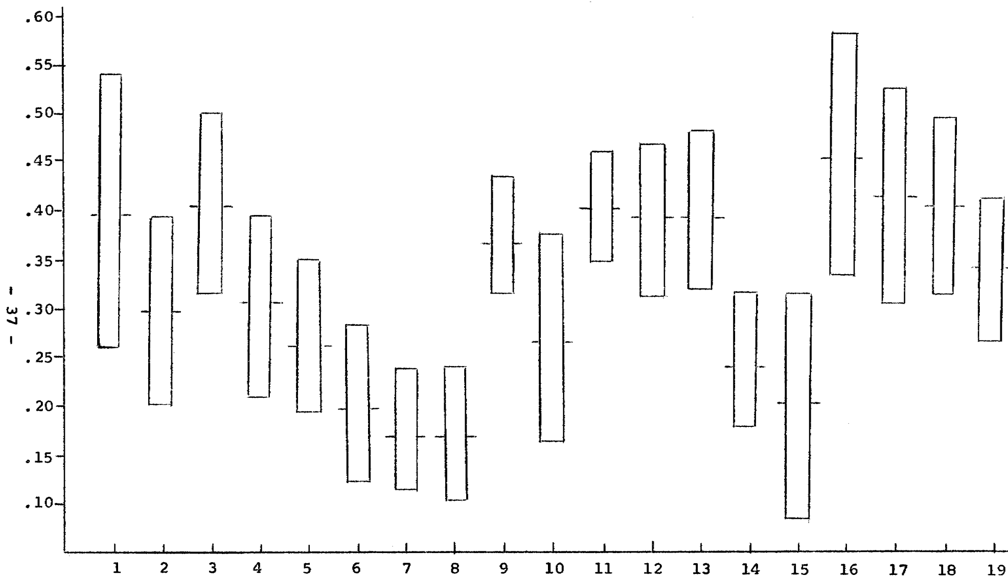
Figure 5. Ninety-five per cent confidence limits for mean of ratio \frac{\text{viable stems}}{\text{dead stems}} , for 19 elderberry transects.
