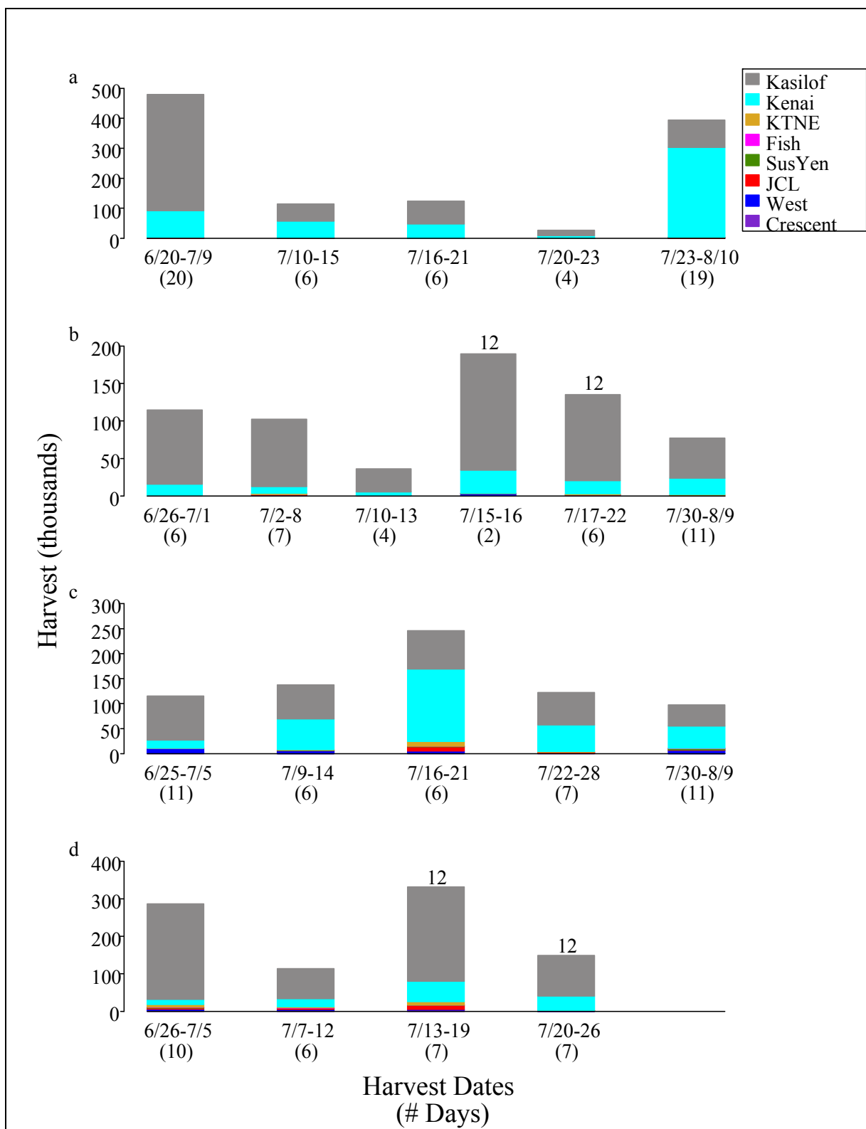
Figure 8.—Estimates of harvest by stock for the Kasilof Section set gillnet fishery (Central District, East Side Subdistrict) from a) 2005, b) 2006, c) 2007, and d) 2008. Numbers above the bars indicate that fishery restrictions during openings (see Table 1).
