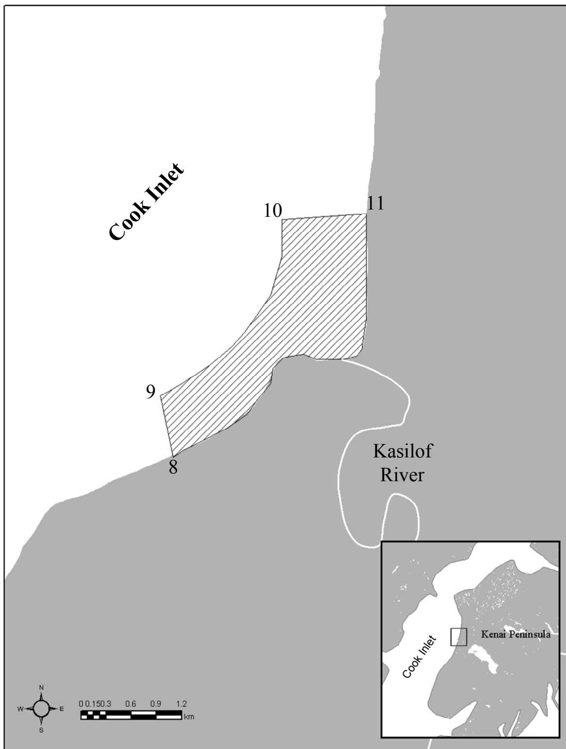
Figure 3.—Map of the mouth of the Kasilof River showing management fishing boundaries for the Kasilof River Special Harvest Area (Central District, East Side Subdistrict) (see Table 1 for description of points).
