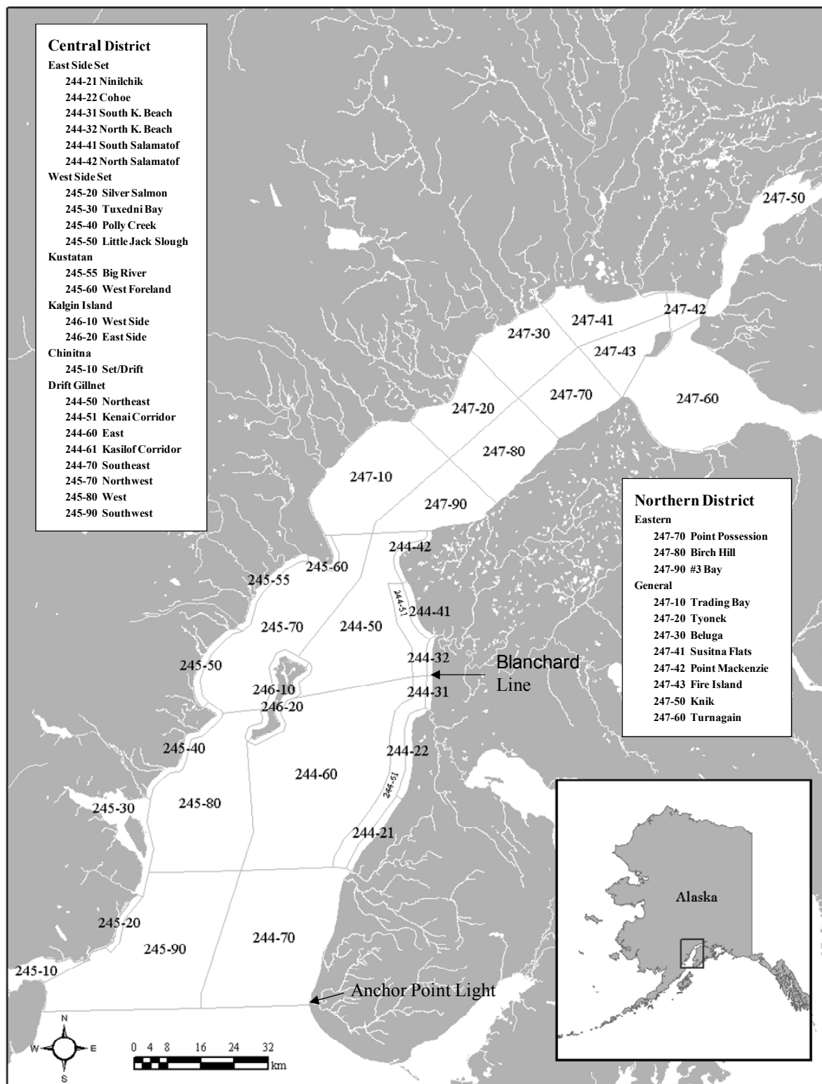
Figure 1.—Map of Upper Cook Inlet showing management fishing boundaries (statistical areas) for subdistricts, sections, and subsections within the Northern and Central Districts for both set and drift gillnet fisheries.
