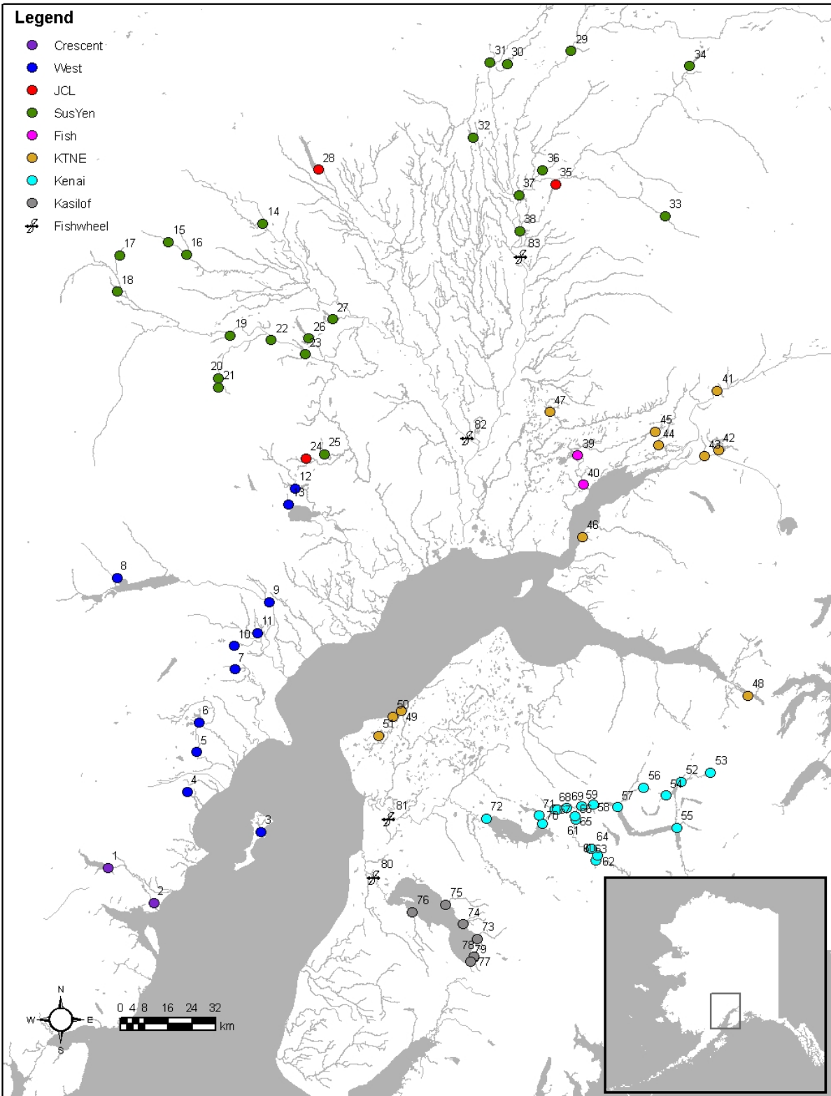
Figure 5.—Sampling locations for sockeye salmon originating for Upper Cook Inlet, Alaska, 1992-2008 used to compile a genetic baseline. Numbers correspond to map numbers on Table 2. Colors for each reporting group and symbols for fish wheels are indicated in the legend.
