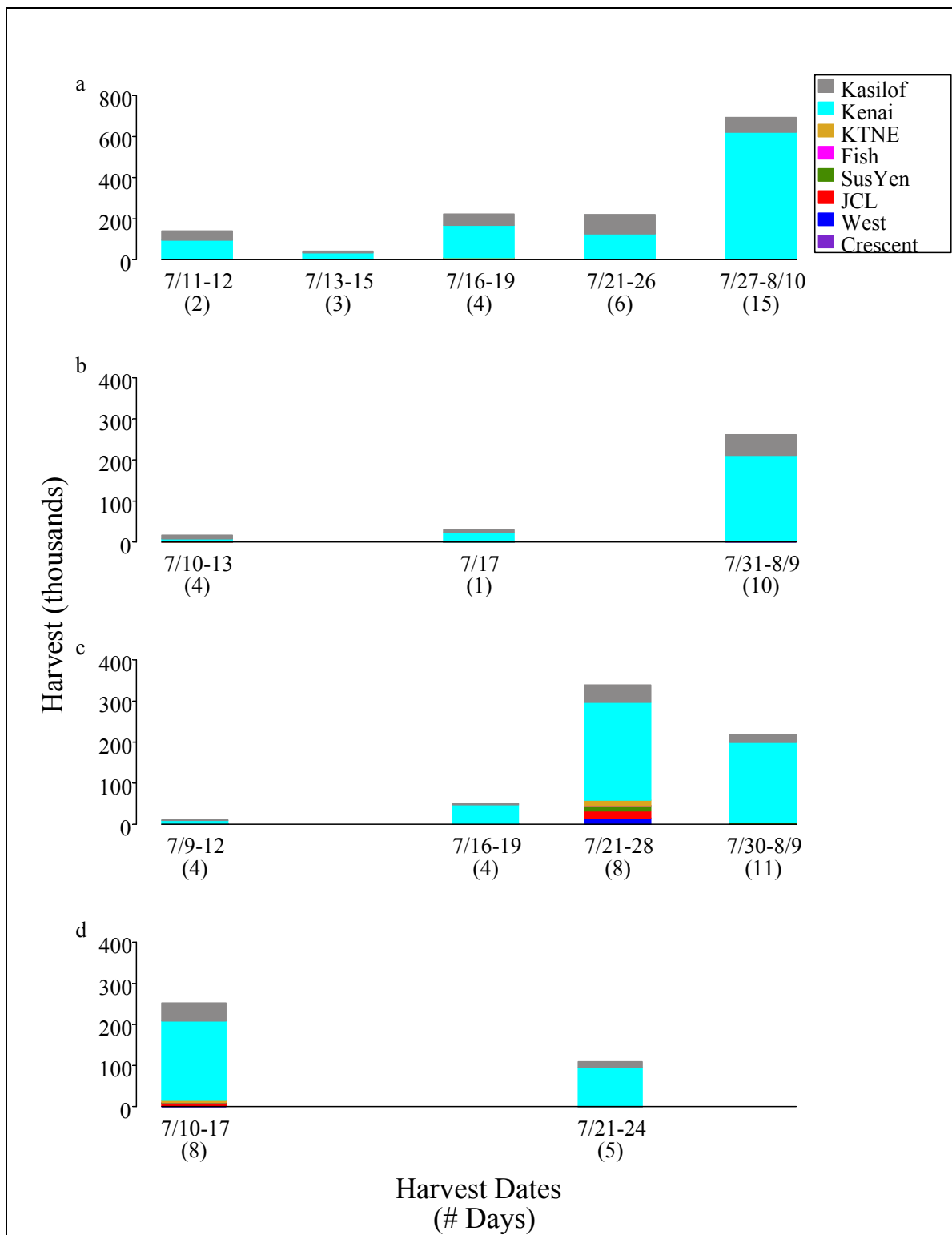
Figure 9.—Estimates of harvest by stock for the Kenai Section set gillnet fishery (Central District, East Side Subdistrict) from a) 2005, b) 2006, c) 2007, and d) 2008.
