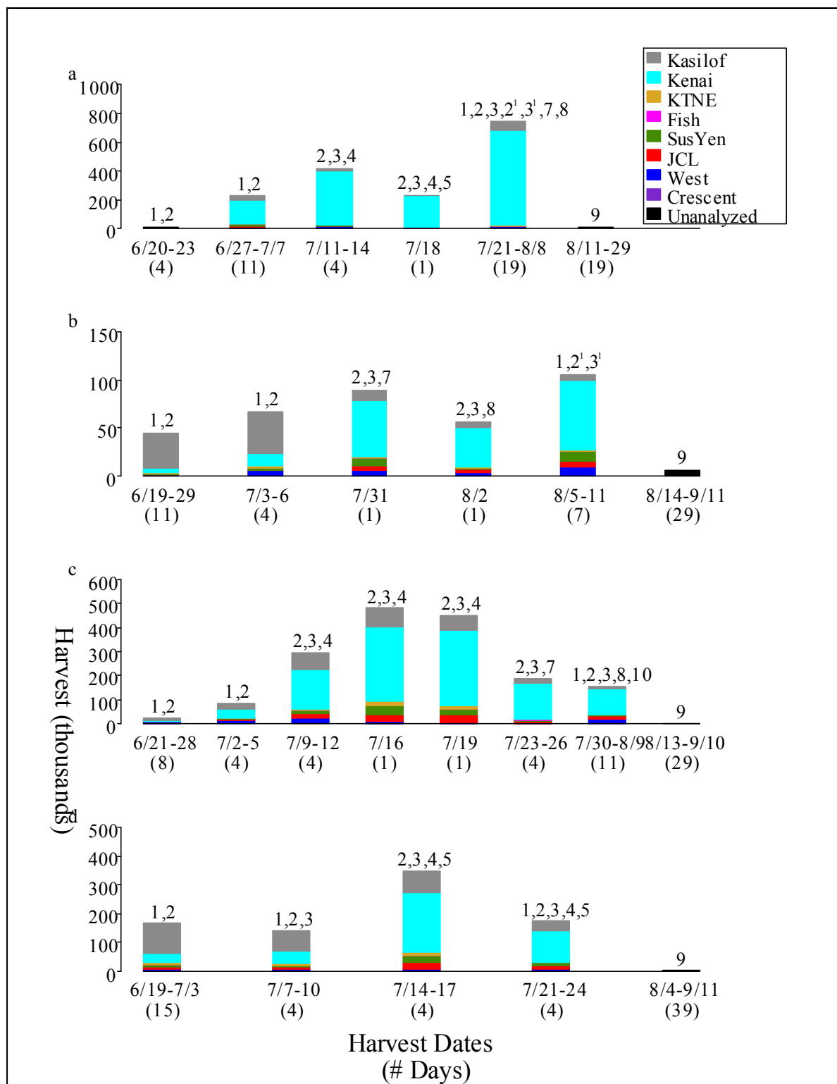
Figure 7.—Estimates of harvest by stock for the Central District drift gillnet fishery (excluding corridor-only periods) from a) 2005, b) 2006, c) 2007, and d) 2008. Numbers above the bars indicate that fisheries were restricted to particular areas (see Tables 1 and 3).
