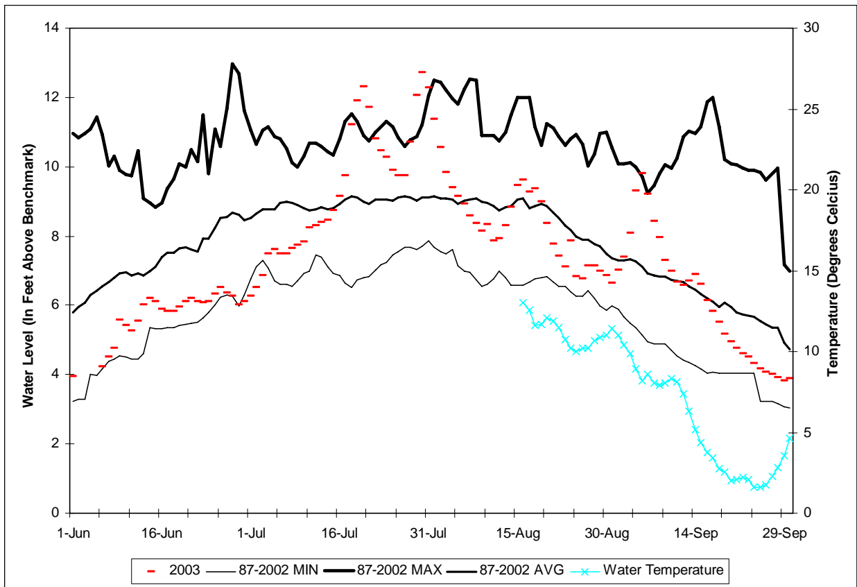
Appendix A1. —Historical Tanana River water levels based on the gage located on the bridge in the community of Nenana, 1987 to 2002 compared to 2003 and subsurface water temperatures taken at the Nenana test fish wheel site in 2003.
