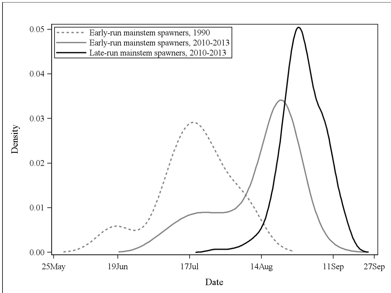
Figure 9.—Kernal density of post spawning mortality date for Chinook salmon with Kenai River mainstem spawning destinations; 1990, 2010–2013.
