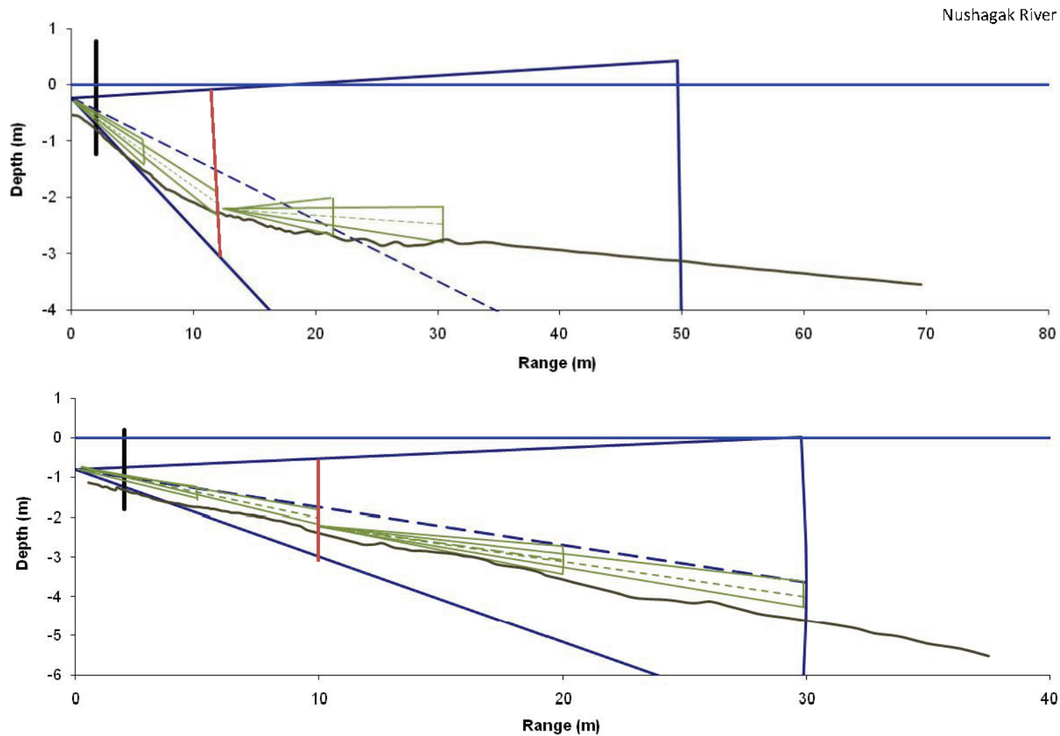
Figure 57.—Nushagak River right-bank (top) and left-bank (bottom) river bottom profiles (wavy line) overlaid with the DIDSON beam (large triangle) and echo-counter beams (small triangles).
