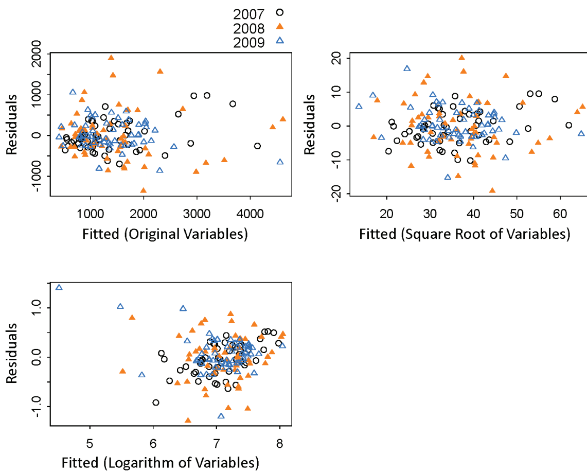
Figure 19.—Residuals from Bendix echo-counter and DIDSON salmon passage estimates, Kasilof River south bank.
