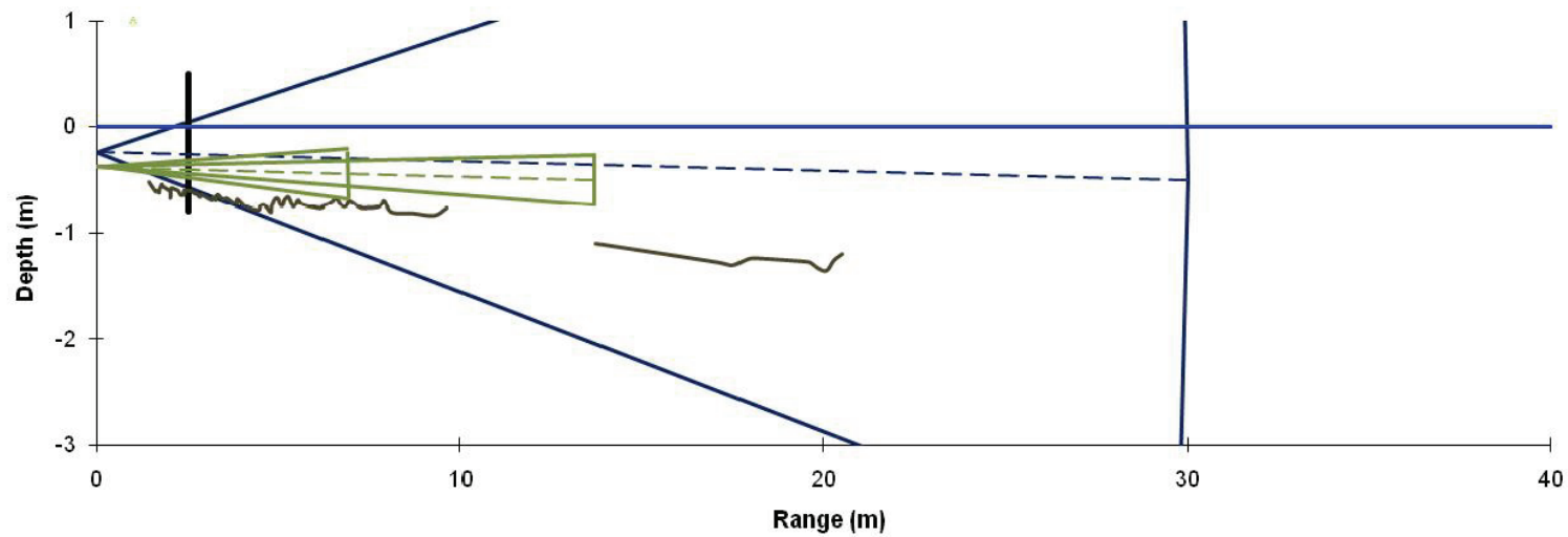
Figure 16.–Kasilof River north bank (top) and south bank (bottom) river bottom profiles (wavy line) overlaid with DIDSON beam (large triangle) and echo-counter beams (small triangles).
