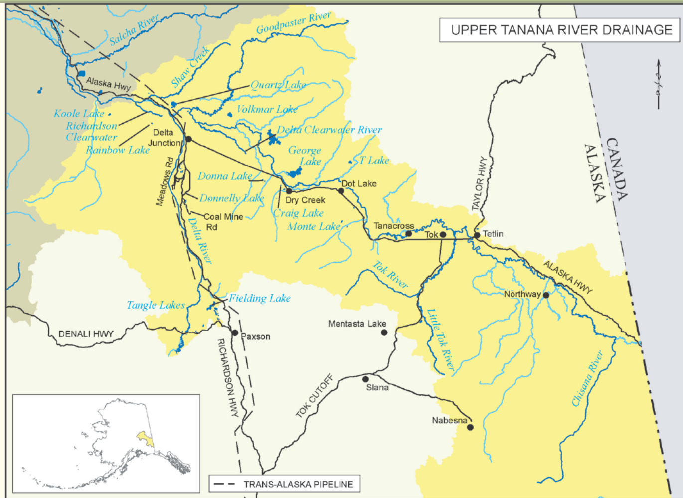
Figure 2.—Map of that portion of the Tanana River drainage located upriver from the Salcha River.
