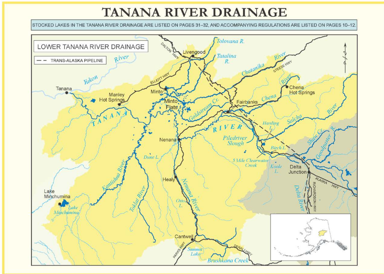
Figure 3.—Map of that portion of the Tanana River drainage located downriver from Shaw Creek.
