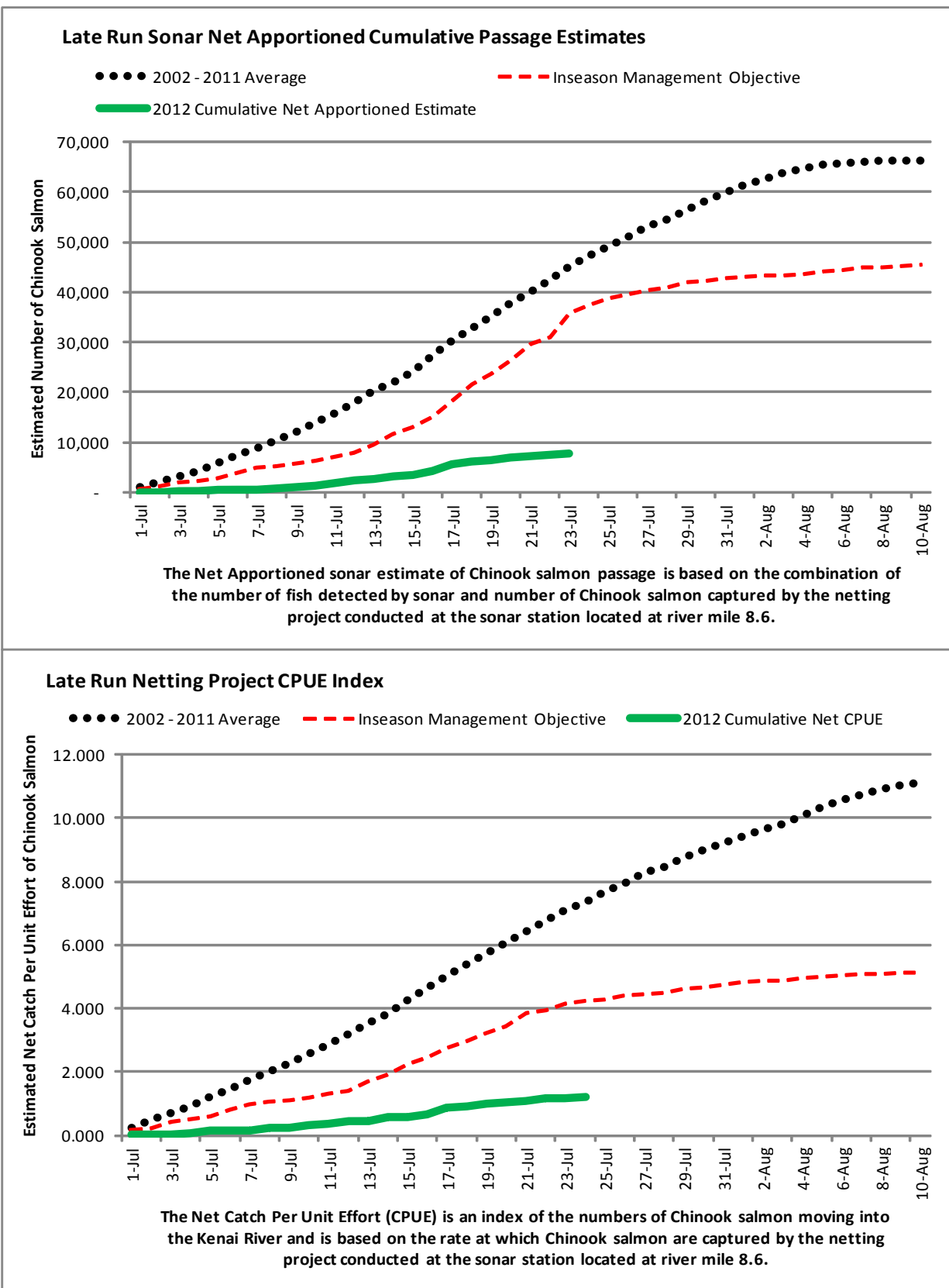
Figure 1. Kenai River late-run Chinook salmon net apportioned sonar estimate and net catch per unit effort (CPUE) index, 2012.
