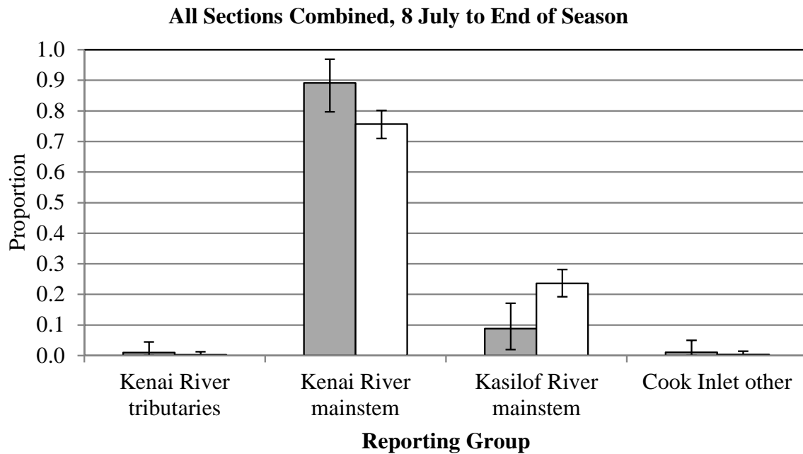
Figure 7.—Age-based (jacks vs. non-jacks) MSA with all 3 years of tissue collections (2010, 2011, and 2013) combined for Kasilof Section, prior to 8 July (top), and all sections combined, 8 July to end of season (bottom).
